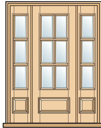
6 Lite #5206 with 3-Lite Sidelite #5216 Doors available 30", 32" & 36" Sidelites available 12"
